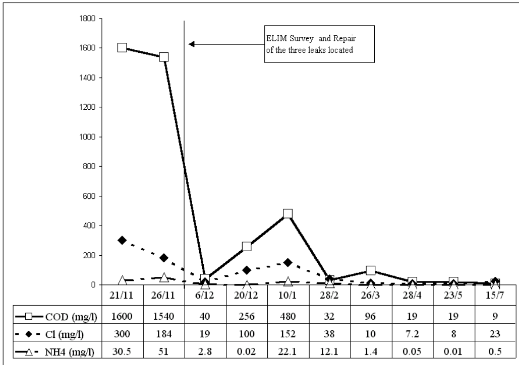
Figure 4: Plot of Groundwater Monitoring Data Indicating High COD and Cl Levels (Note: pollutant levels decreased after leaks located with ELIM were repaired)
