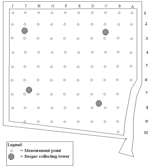
Figure 2. Drawing Showing Survey Grid
