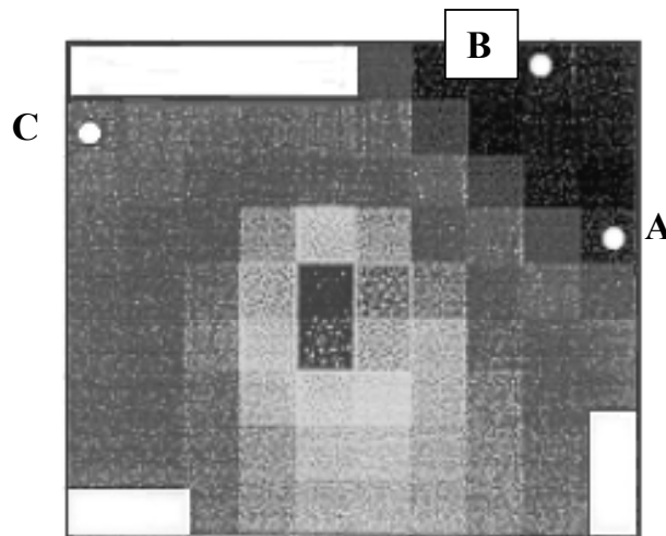
Figure 3: Plot of ELIM data collected at the landfill showing three leak signals (Position "A" 63 cm x 31 cm tear. Position "B" 10 cm x 5 cm hole. Position "C" 5 cm X 3 cm hole)
